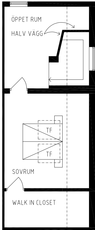
PLAN 3 TR
